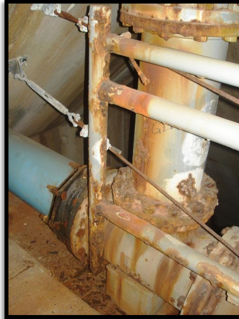
Corrosion to pipe and handrails; replaced pipe to left of valve
