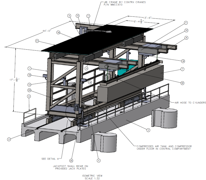
Trolley/Winch Cart
