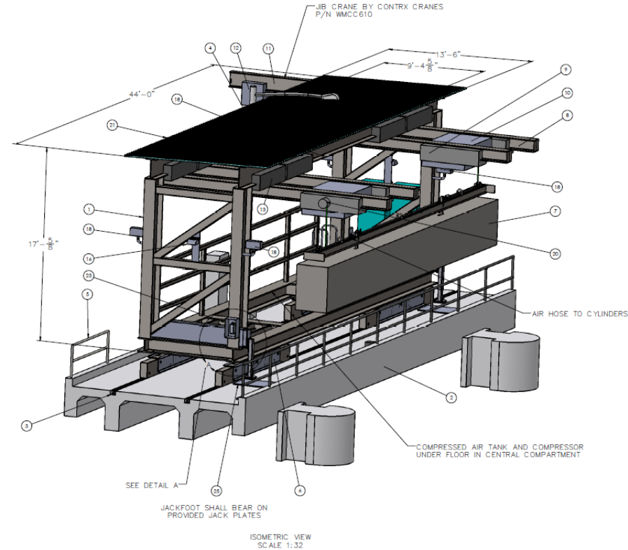
Trolley/Winch Cart
